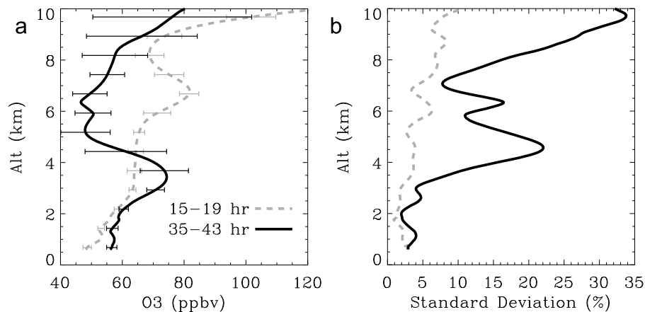
Figure 9. Variability of the ozone lidar measurements in Figure 5. (a) Average ozone of the 10-min lidar profiles and its 1- \sigma standard deviation. The gray dashed line represents the observation duration from 0300 to 0645 28 April ( \sim 15–19 h after the intrusion) and the black solid line represents the observation duration from 2230 28 April to 0630 29 April ( \sim 35–43 h after the intrusion). The interval of the standard deviation is 750 m which represents the vertical resolution of the lidar measurements. (b) The 1- \sigma standard deviation of the two periods in unit of percentage.
